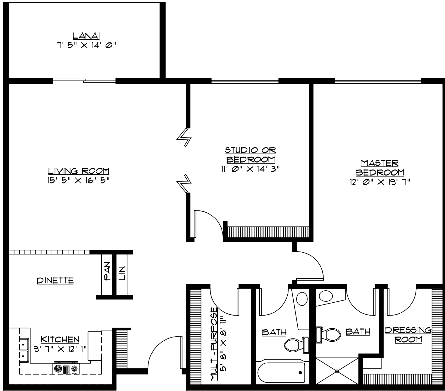
DINETTE " A " 1200 SQ. FT. 2 BEDROOMS AND 2 BATHS
